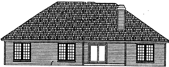
REAR ELEVATION
