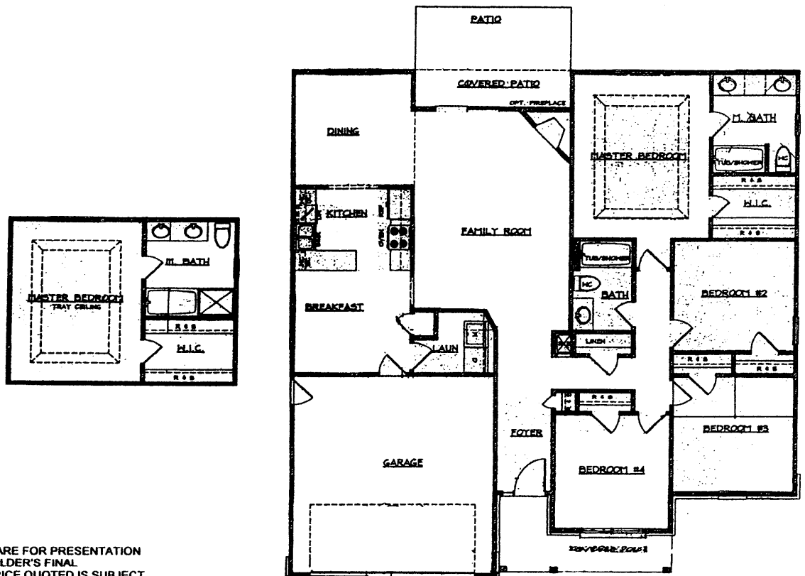
FLOOR PLAN- 106
